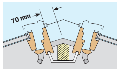
Section, top, if a back-to-back solution is requested
