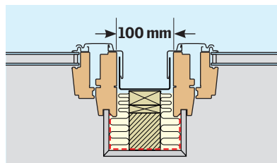
Section between roof windows
