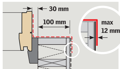
Section, side frame
